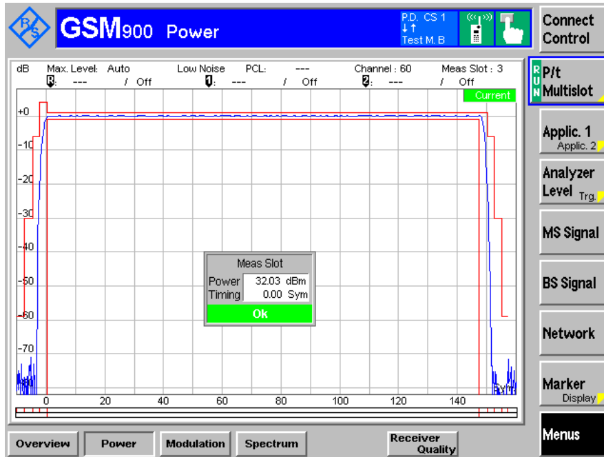
Normal Condition ( \gamma=3 ), Middle Channel, 902.0 MHz
