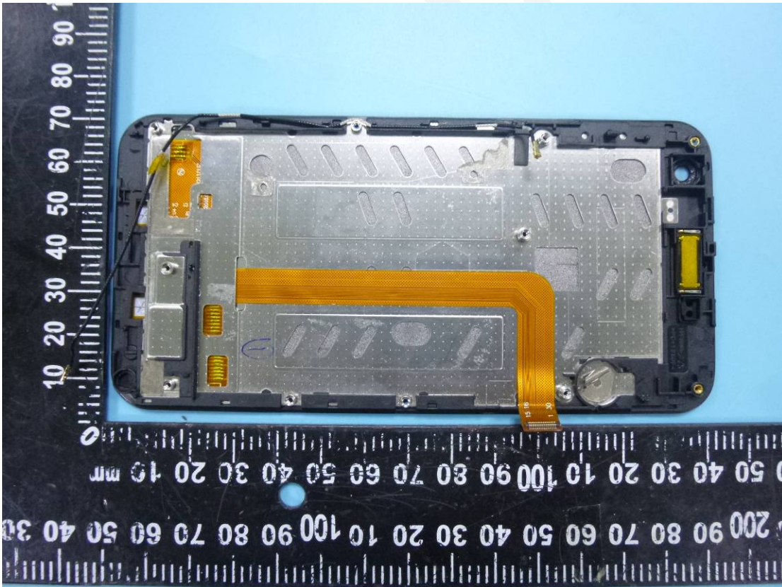
A.8 EUT-Bottom view of LCM
