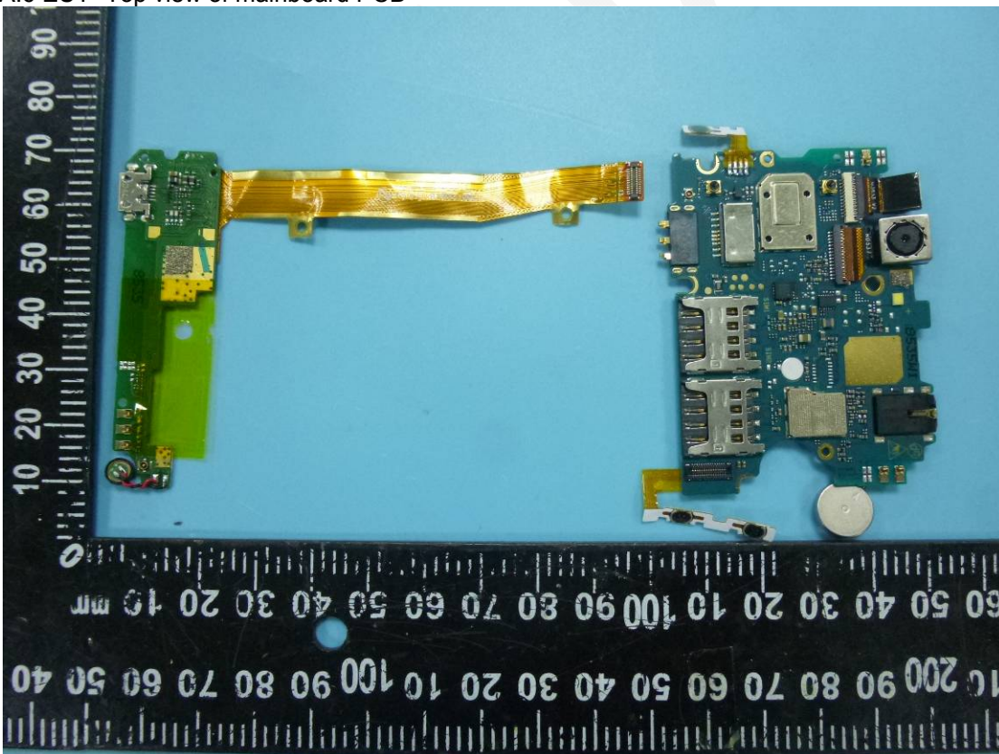
A.6 EUT- Top view of mainboard PCB
