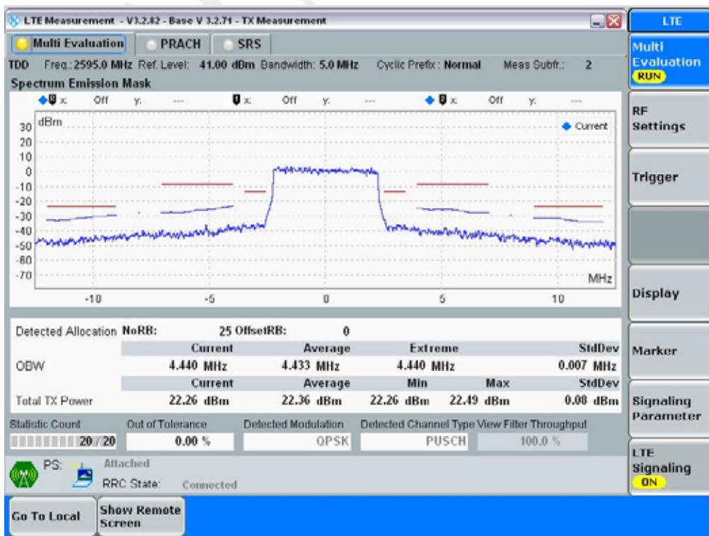
Band 38_5 MHz_QPSK_RB25#0_Middle
