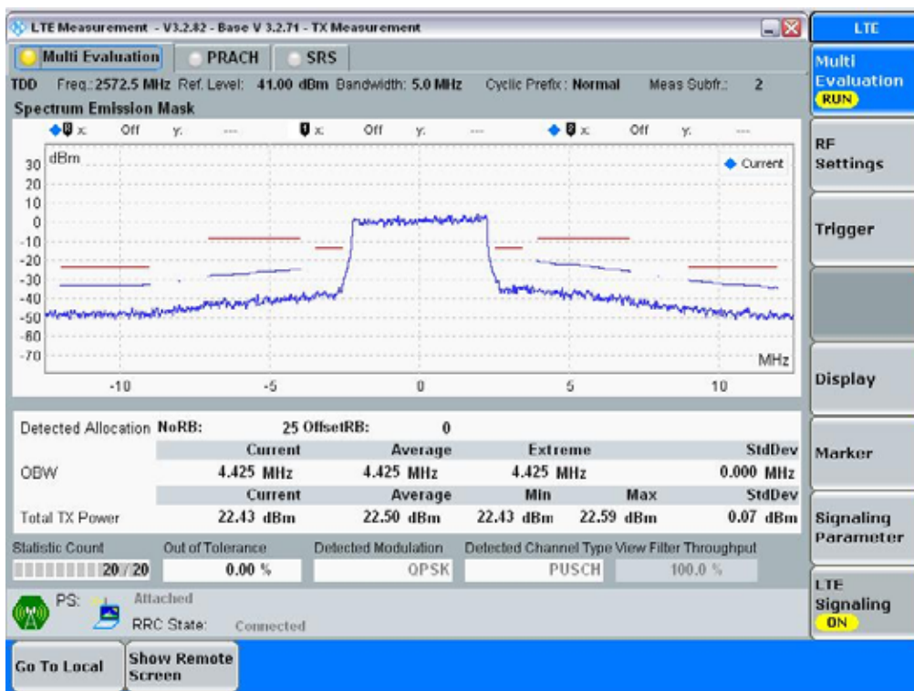
Band 38_5 MHz_QPSK_RB25#0_Low
