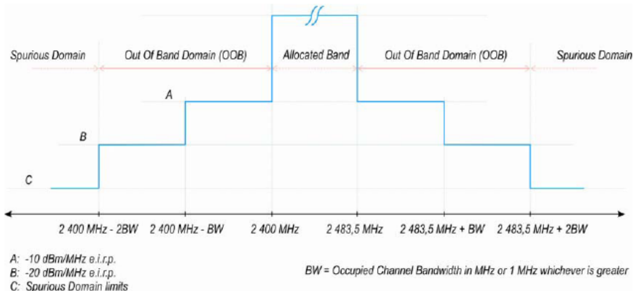
Figure 3: Transmit mask
