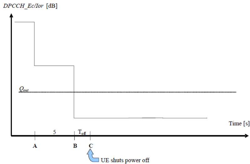
Figure 4.2.11.2-1: Conditions for out-of-synchronization handling in the UE
